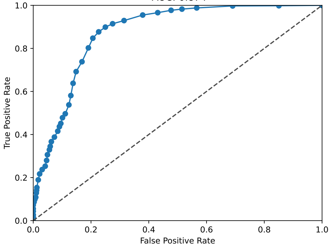
SOX11 ROC Curve AUC: 0.874
