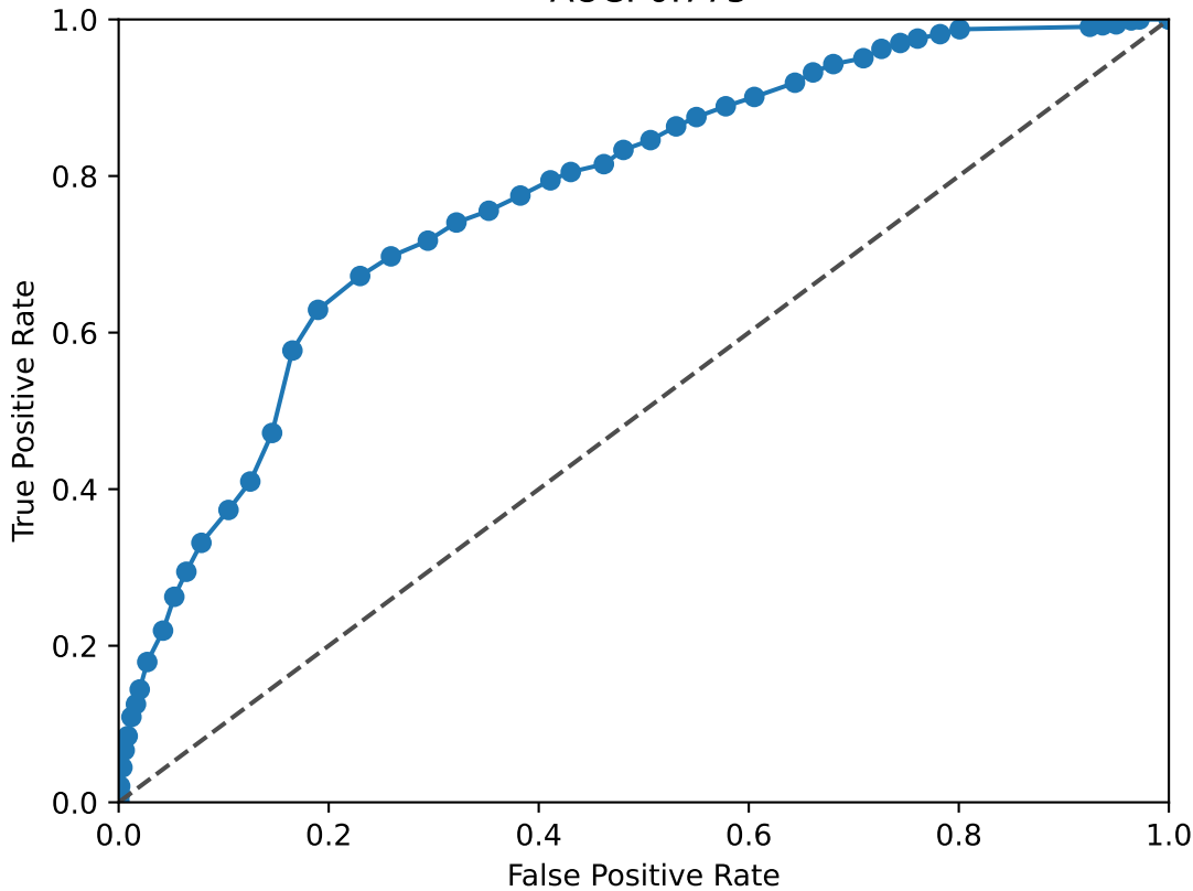
EPCAM ROC Curve AUC: 0.775
