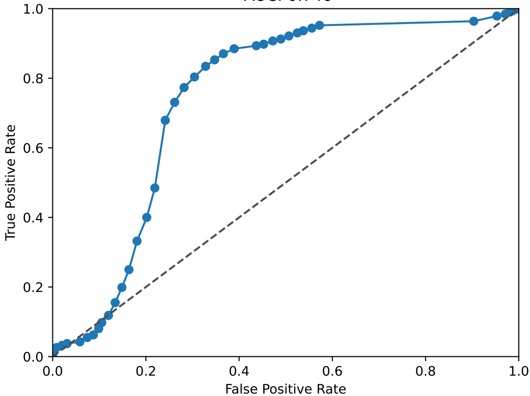
ETS1 ROC Curve AUC: 0.746
