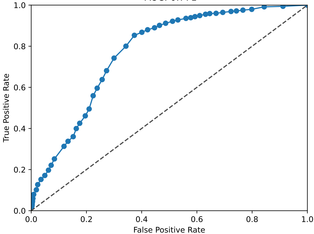
HES1 ROC Curve AUC: 0.771
