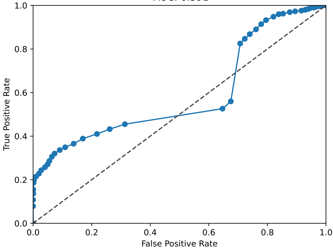
JUNB ROC Curve AUC: 0.591
