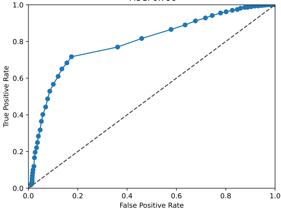
JUN ROC Curve AUC: 0.796
