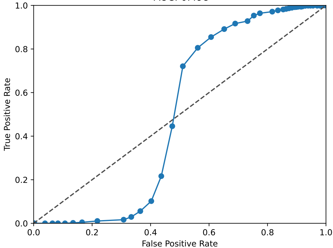
KMT2A ROC Curve AUC: 0.498
