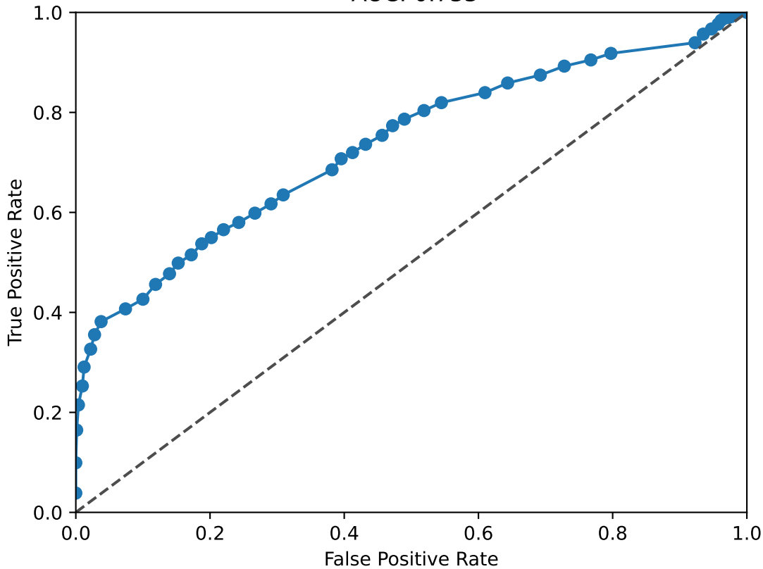
LMX1B ROC Curve AUC: 0.733
