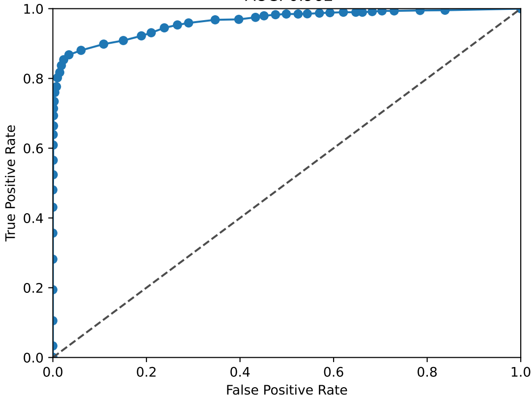
NFIB ROC Curve AUC: 0.962
