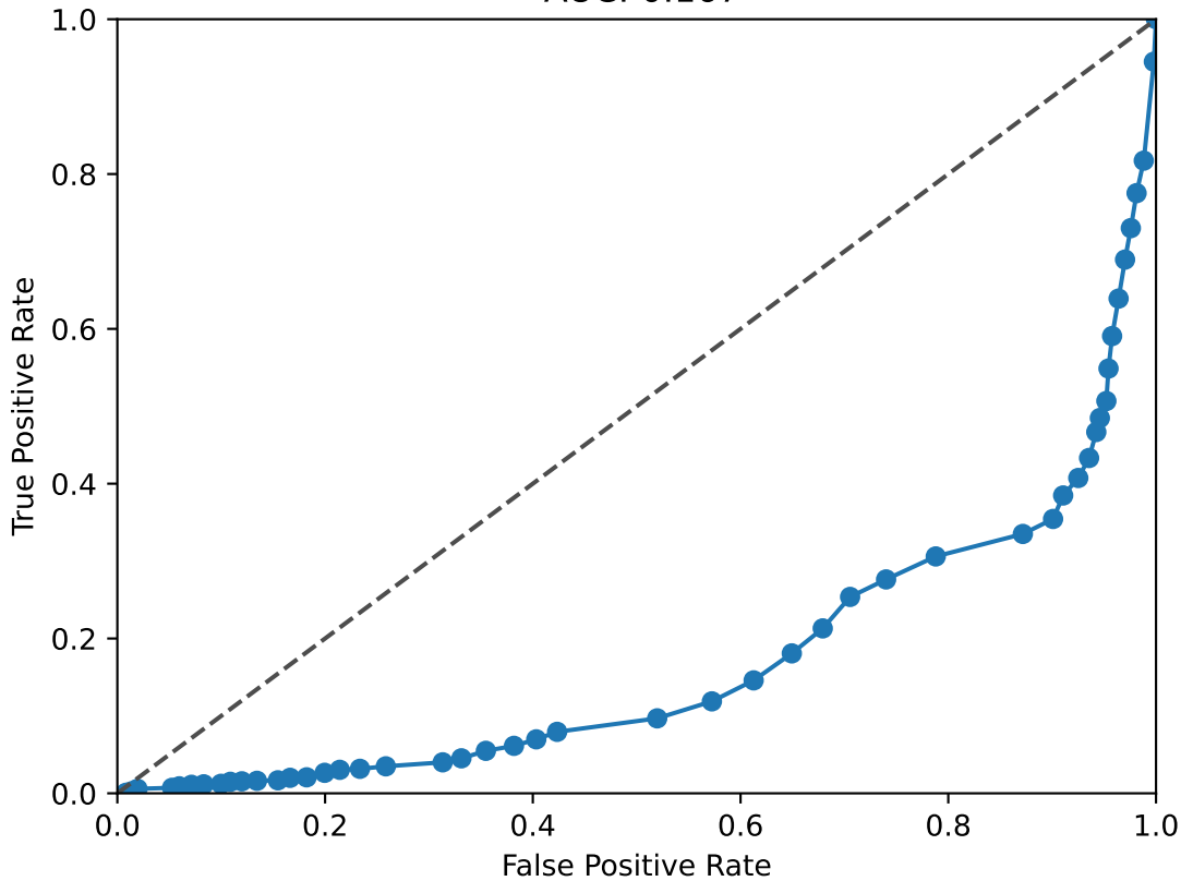
NFIX ROC Curve AUC: 0.167
