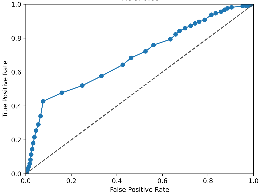
PBX1 ROC Curve AUC: 0.69
