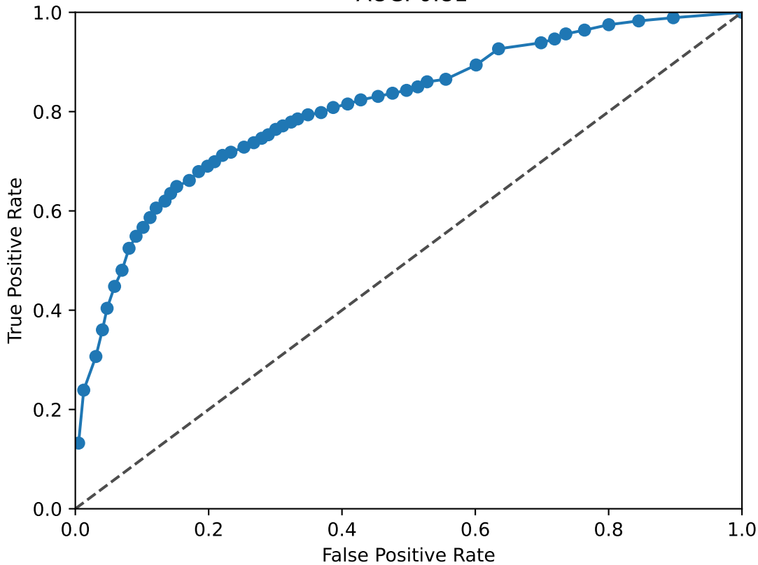
RORA_RORB ROC Curve AUC: 0.81
