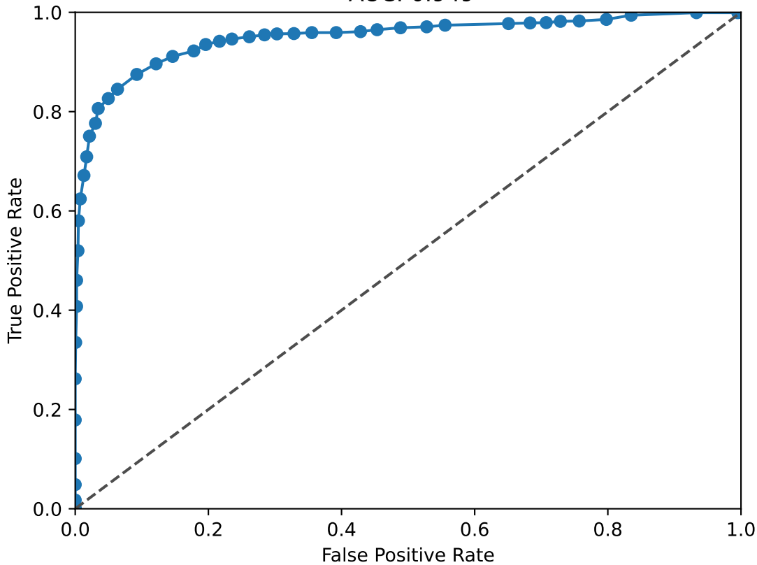
SIX4 ROC Curve AUC: 0.949
