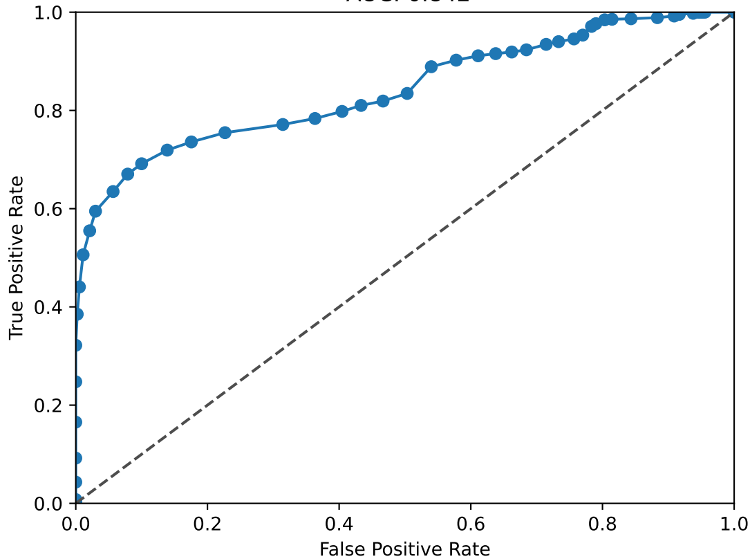
CUX2 ROC Curve AUC: 0.842
