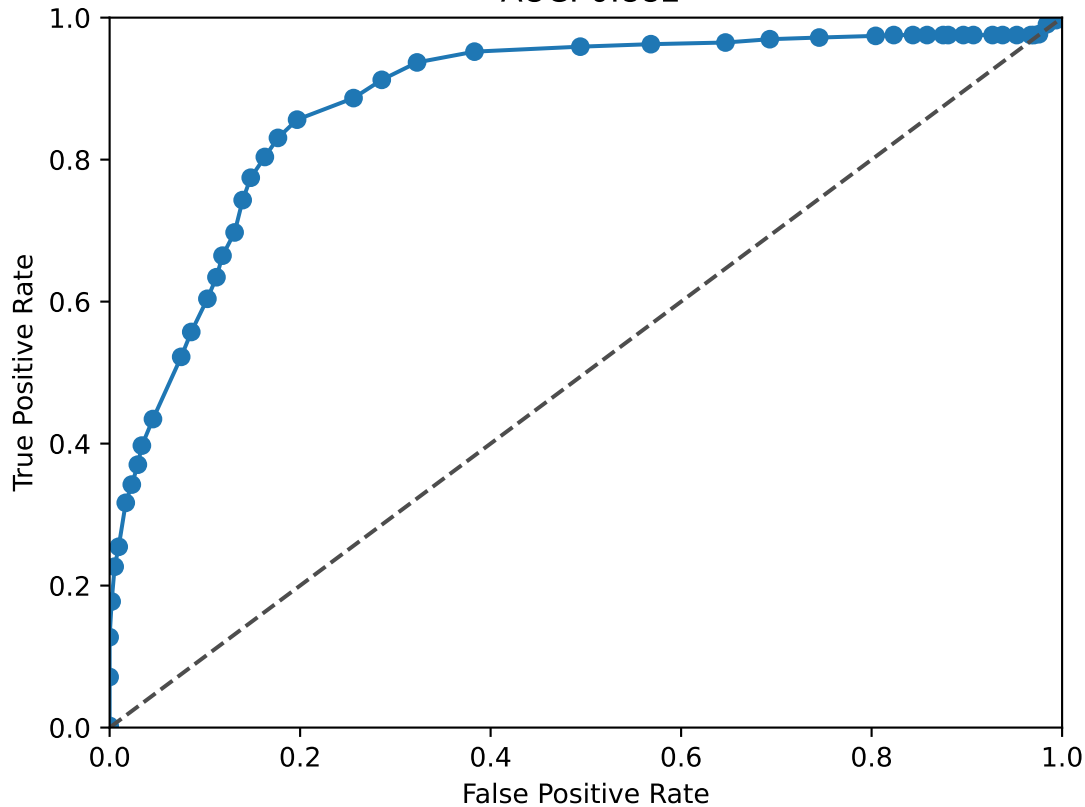
EGR1 ROC Curve AUC: 0.882
