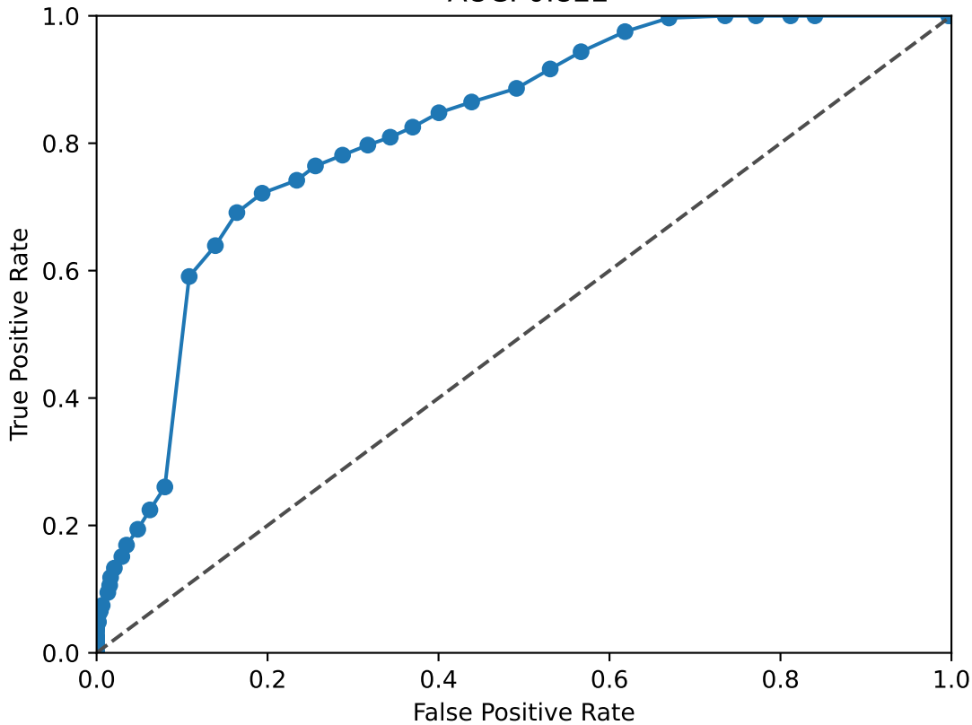
ICAM1 ROC Curve AUC: 0.822
