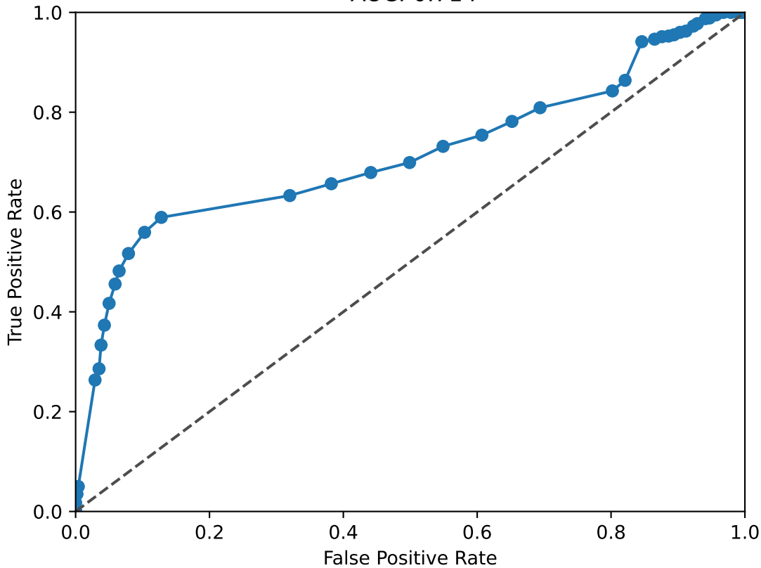
JUNB ROC Curve AUC: 0.714
