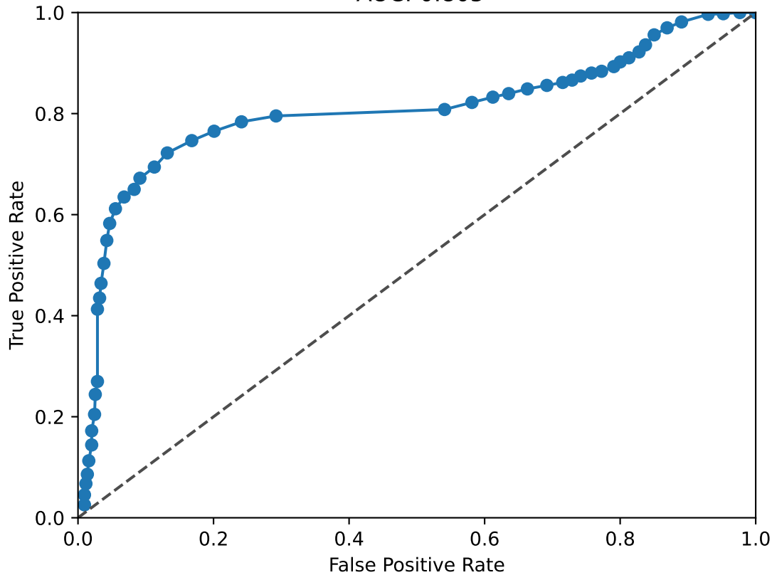
JUN ROC Curve AUC: 0.805
