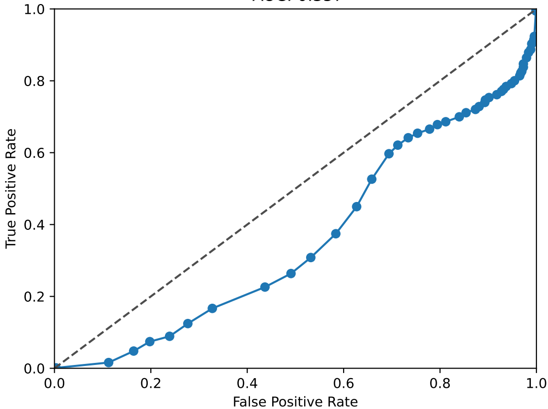
KMT2A ROC Curve AUC: 0.357
