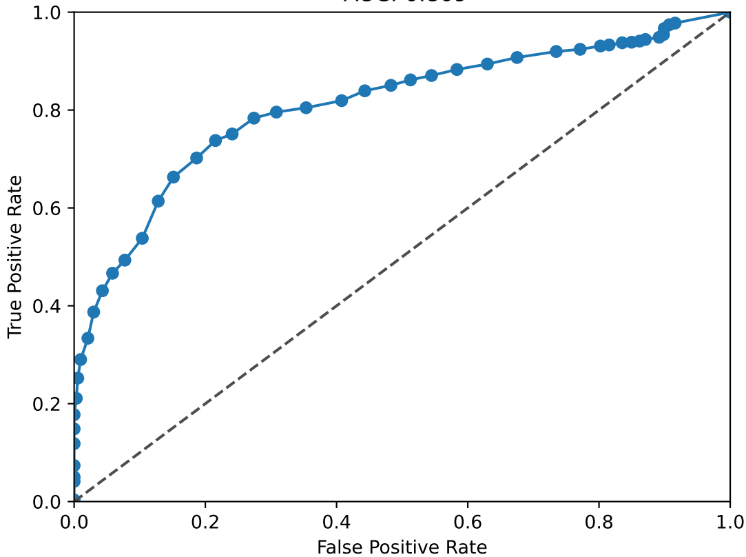
NFIA ROC Curve AUC: 0.809
