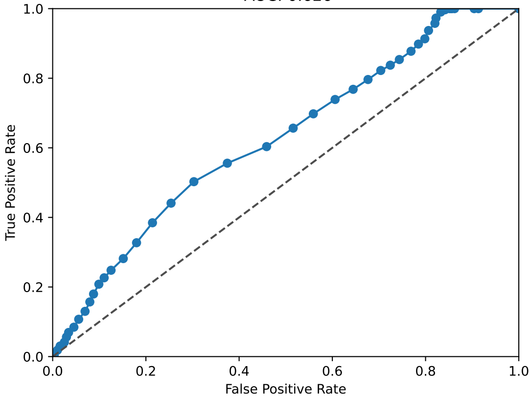
NFIB ROC Curve AUC: 0.626
