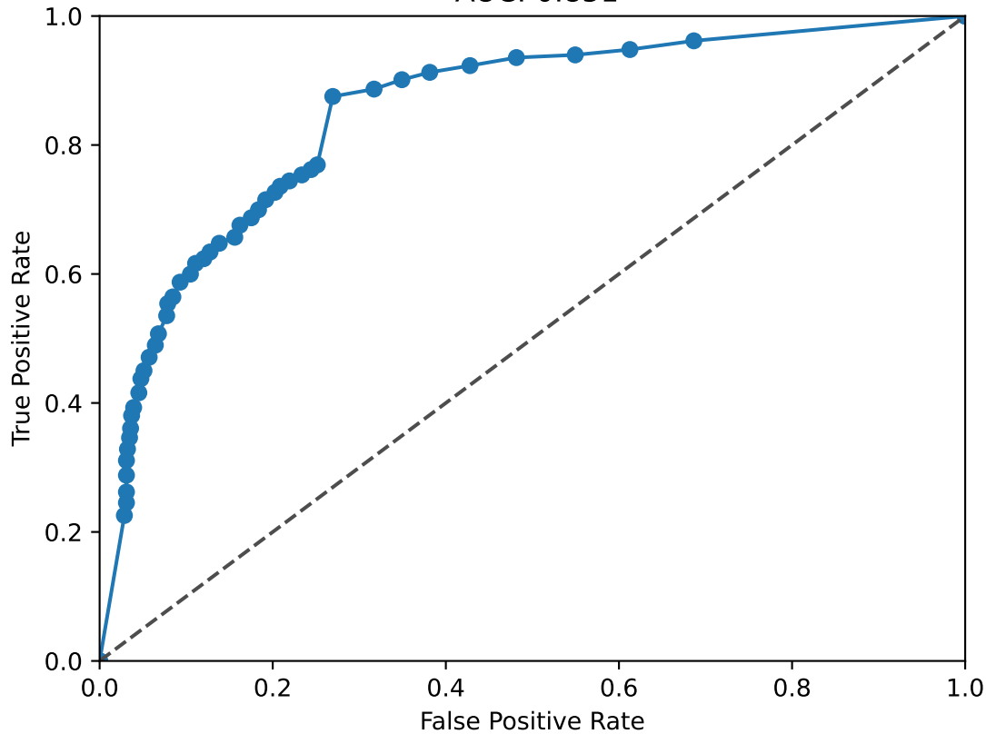
PROX1 ROC Curve AUC: 0.851
