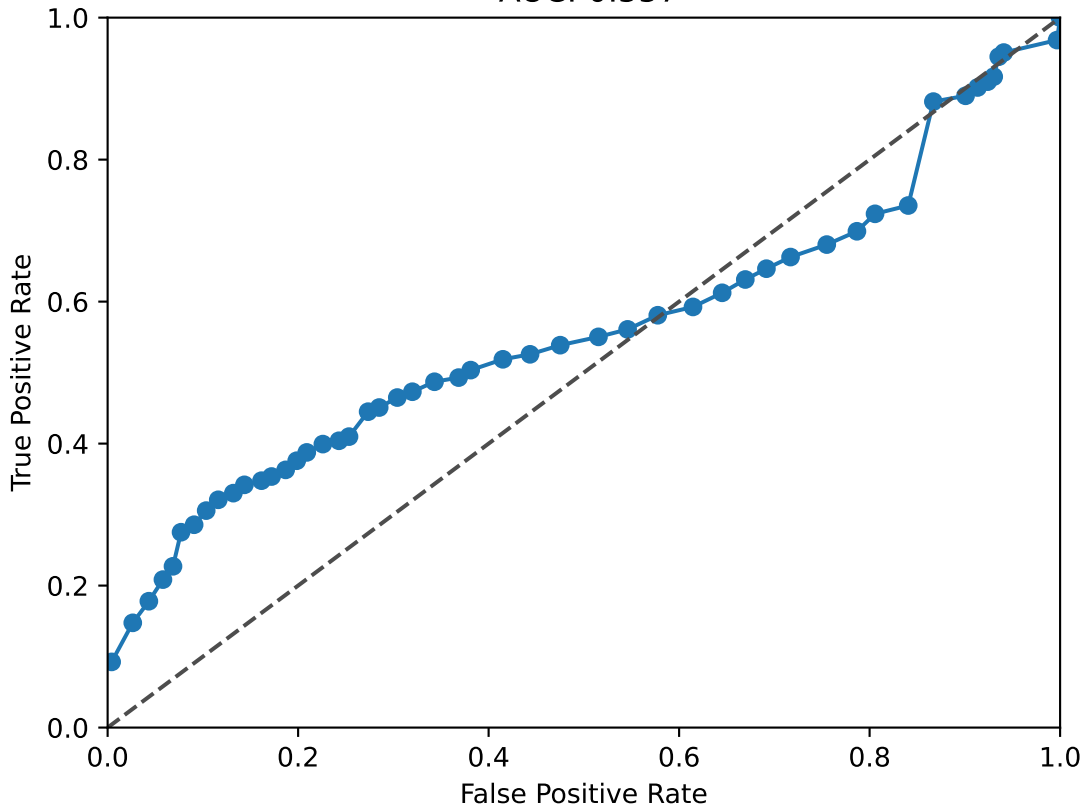
RORA_RORB ROC Curve AUC: 0.557
