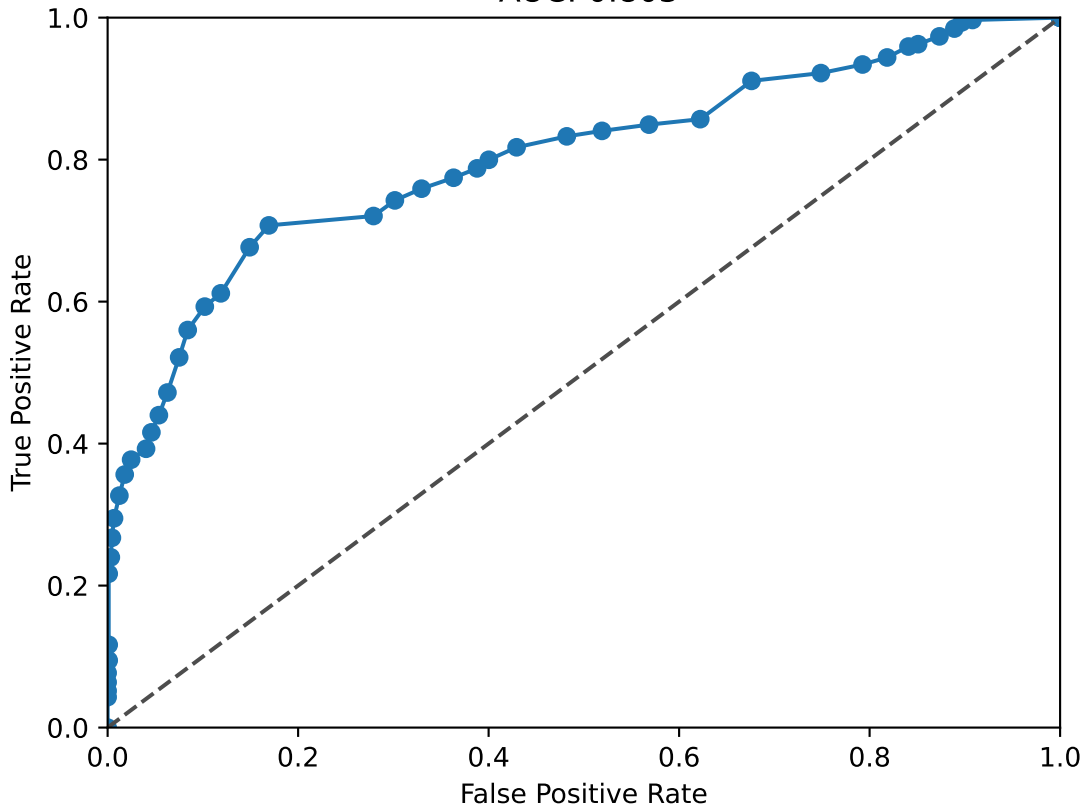
STAT2 ROC Curve AUC: 0.803
