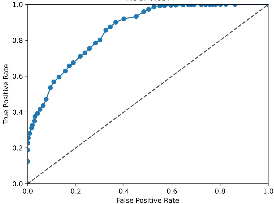
TEAD1 ROC Curve AUC: 0.857
