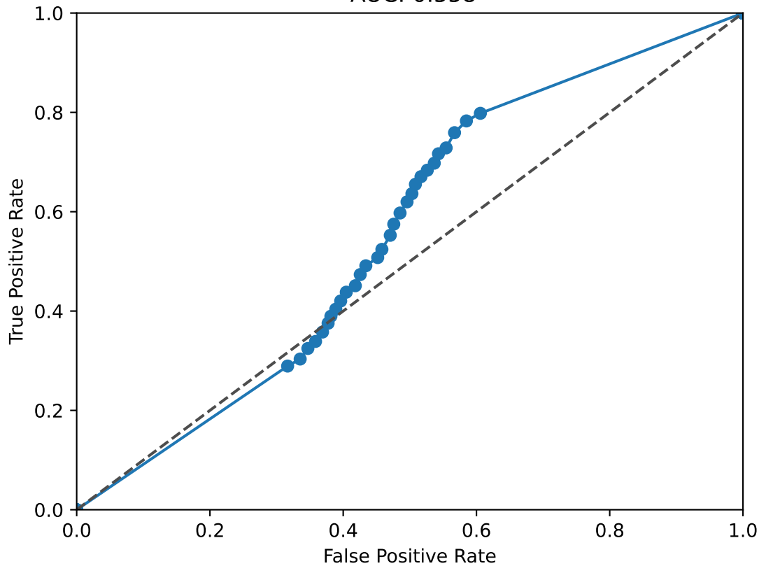
THR B ROC Curve AUC: 0.558
