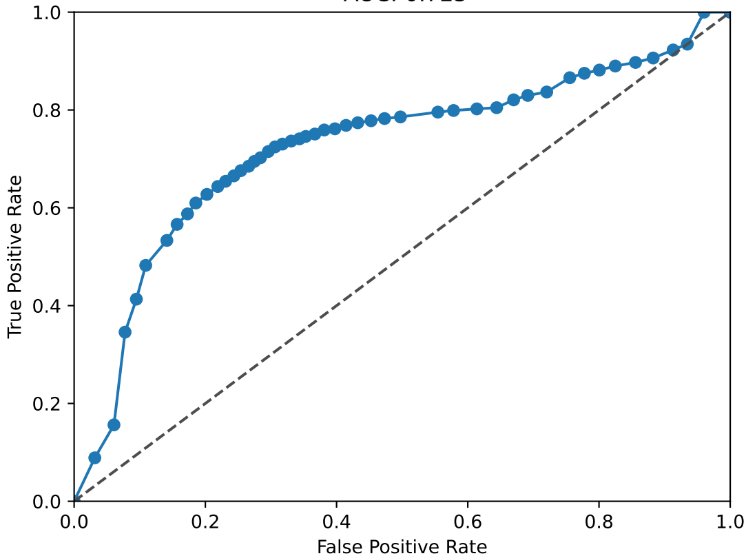
BACH1 ROC Curve AUC: 0.725
