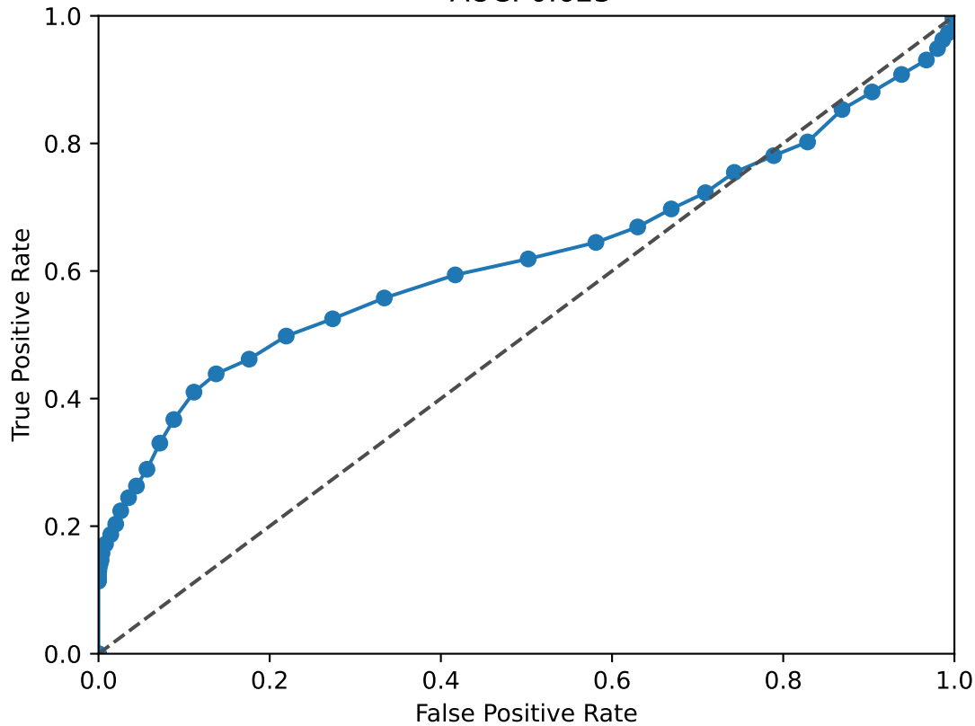
FOS ROC Curve AUC: 0.623
