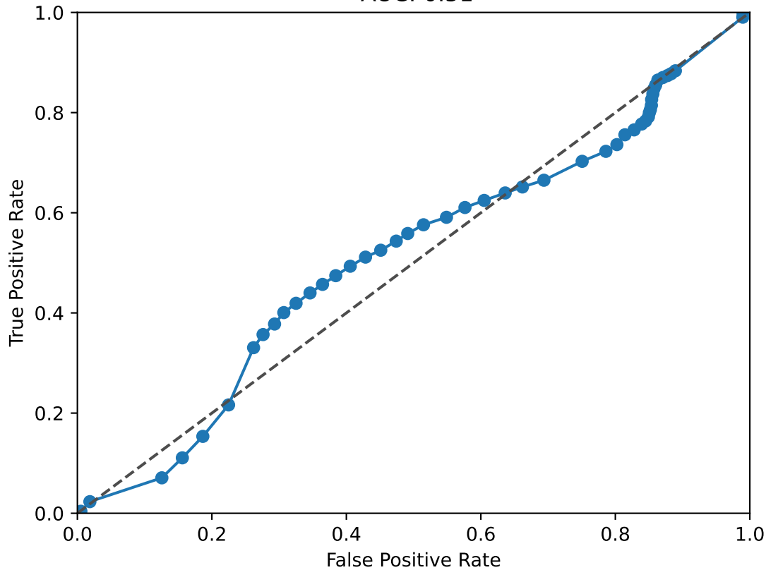
GRHL2 ROC Curve AUC: 0.51
