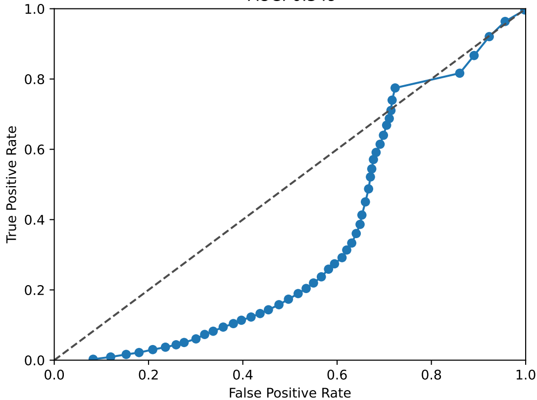
HSF2 ROC Curve AUC: 0.349
