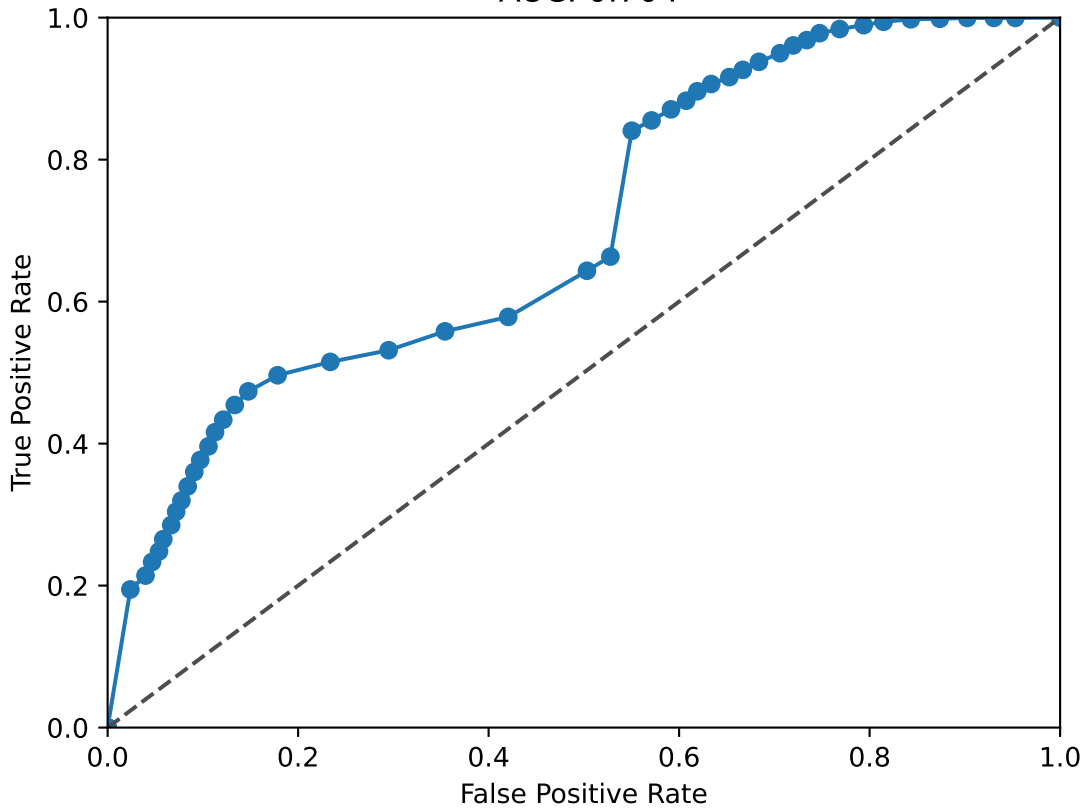
JUNB ROC Curve AUC: 0.704
