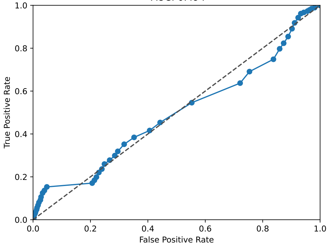
NFIX ROC Curve AUC: 0.494
