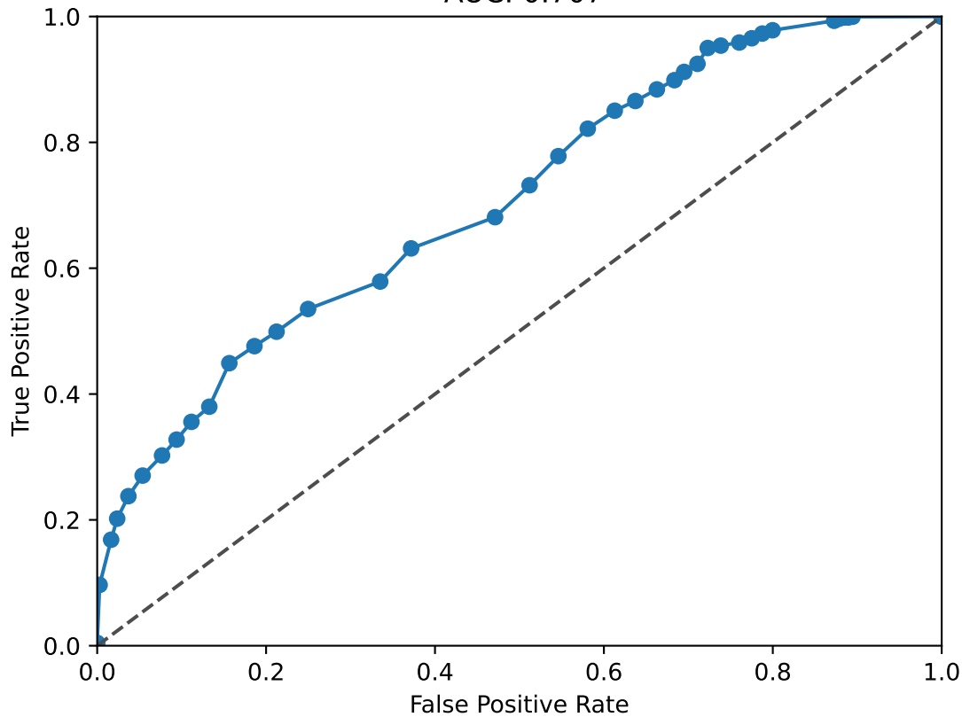
PBX1 ROC Curve AUC: 0.707
