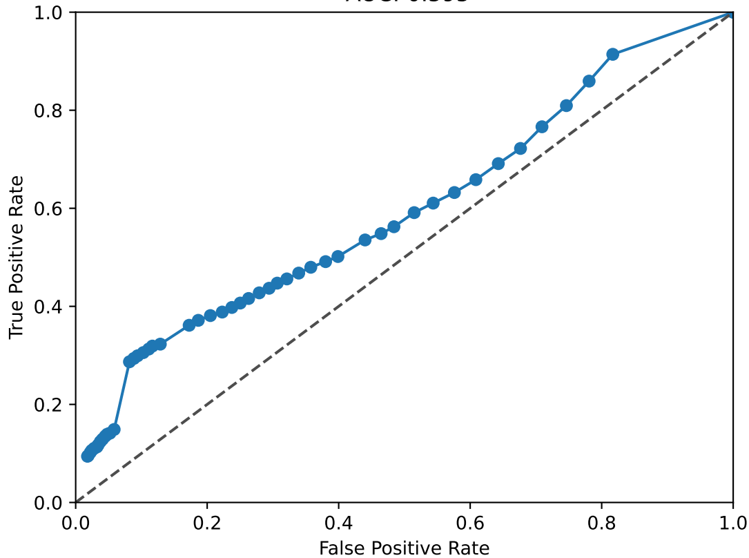
REST ROC Curve AUC: 0.595
