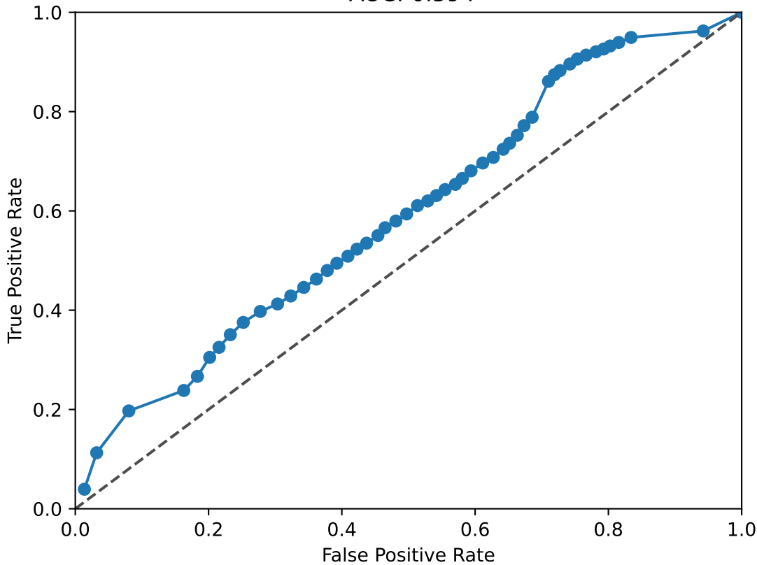
RORA_RORB ROC Curve AUC: 0.594
