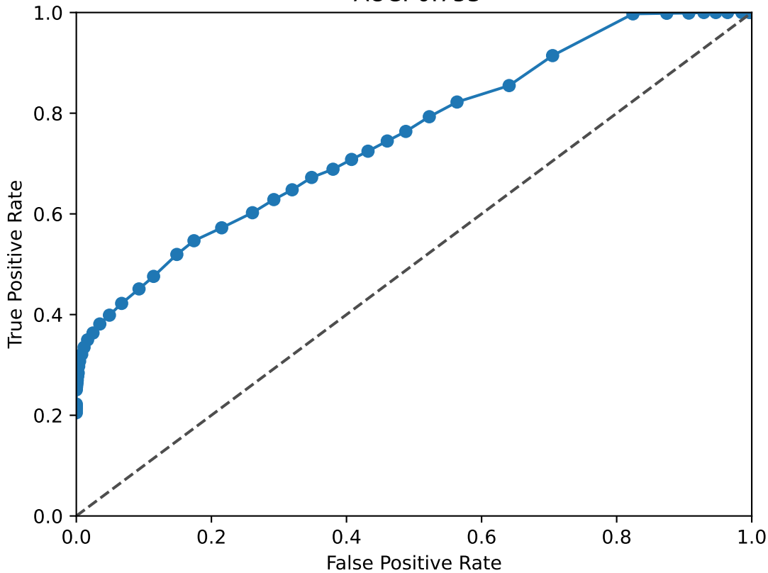
RUNX1 ROC Curve AUC: 0.753
