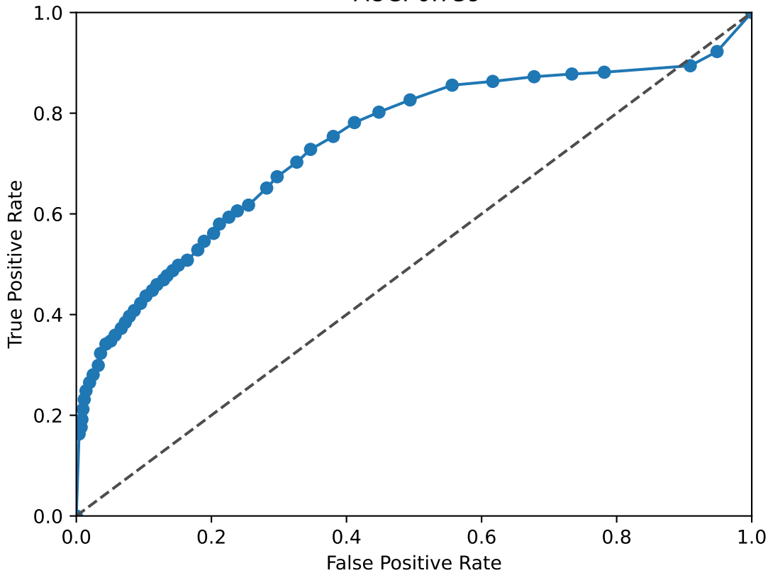
SIX1 ROC Curve AUC: 0.739
