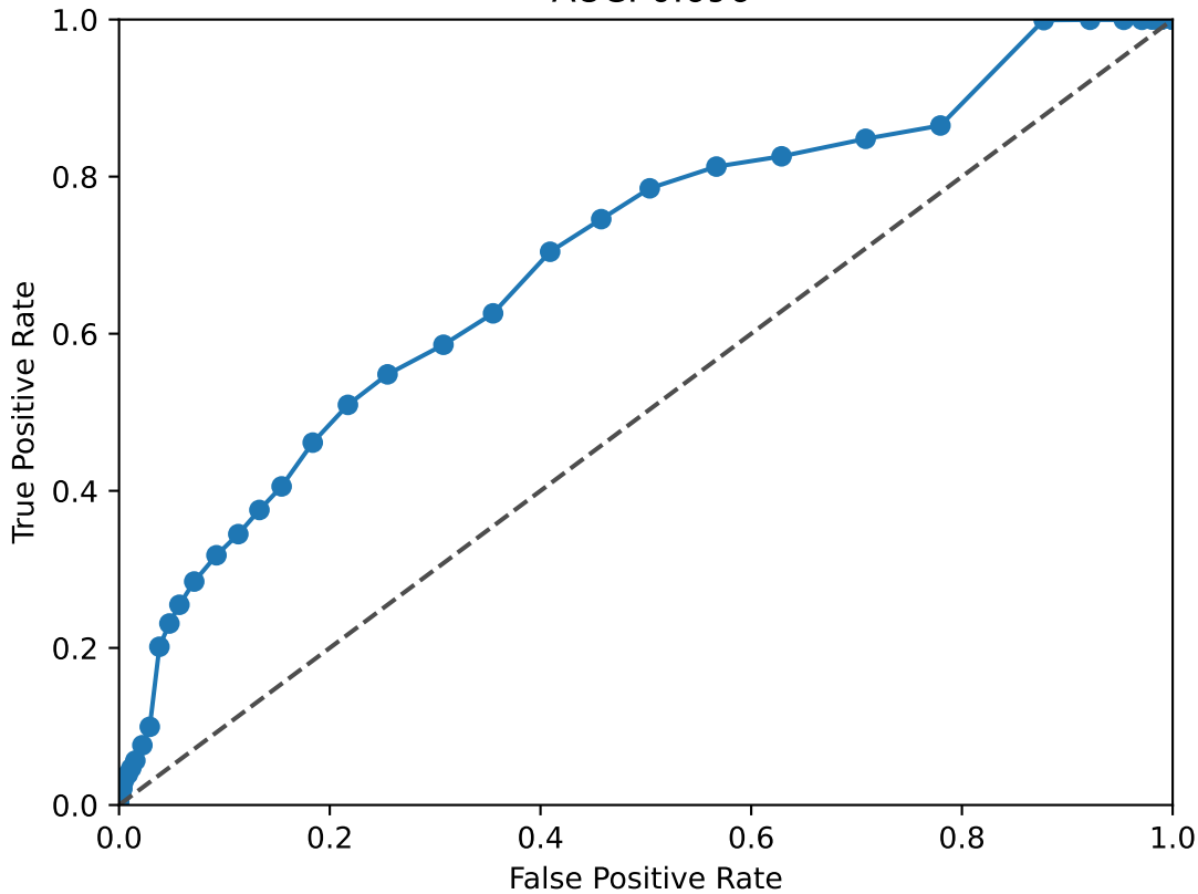
STAT2 ROC Curve AUC: 0.696
