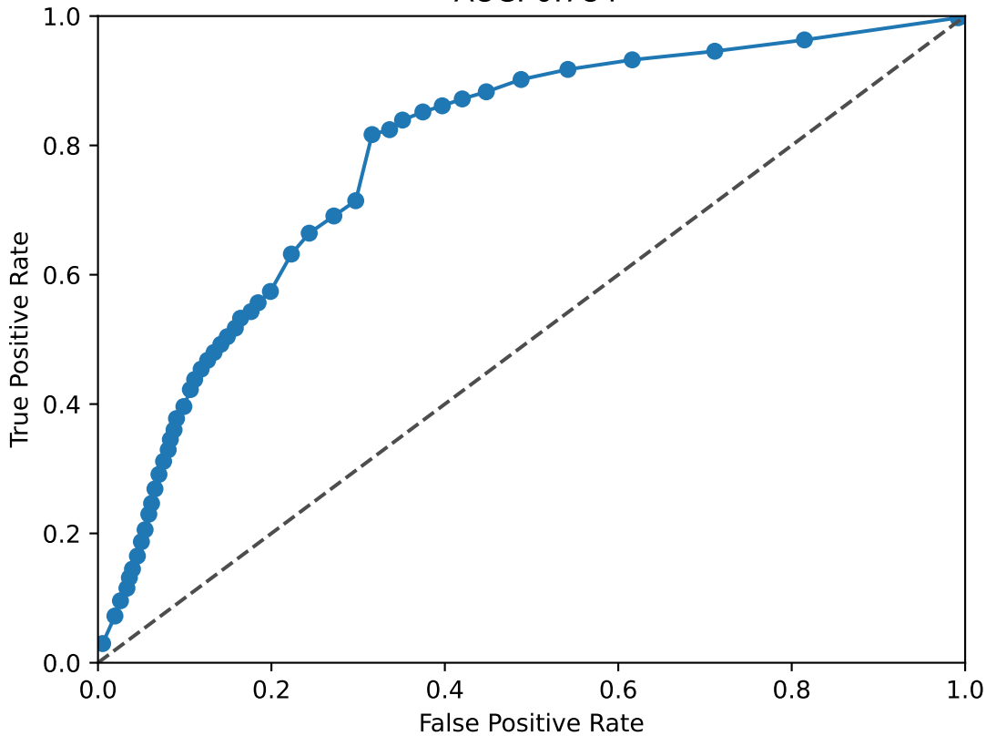
TCF7L2 ROC Curve AUC: 0.784
