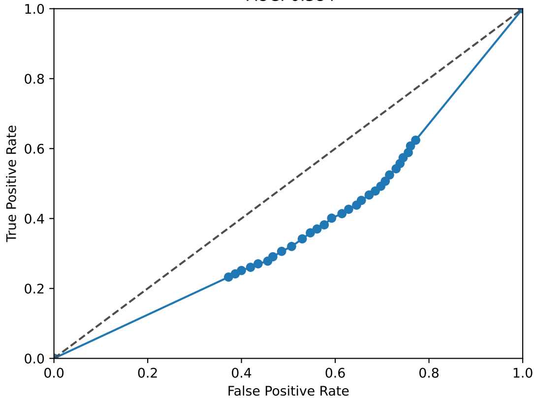
THRB ROC Curve AUC: 0.384
