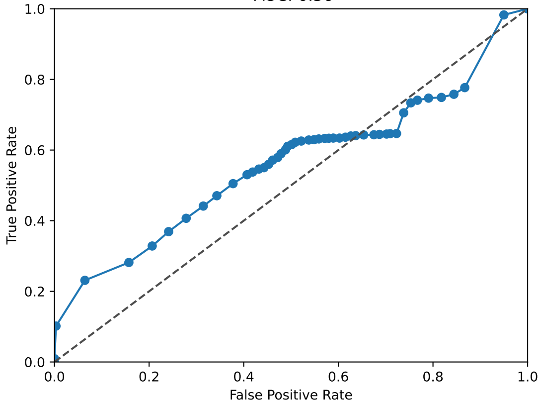
BACH1 ROC Curve AUC: 0.56
