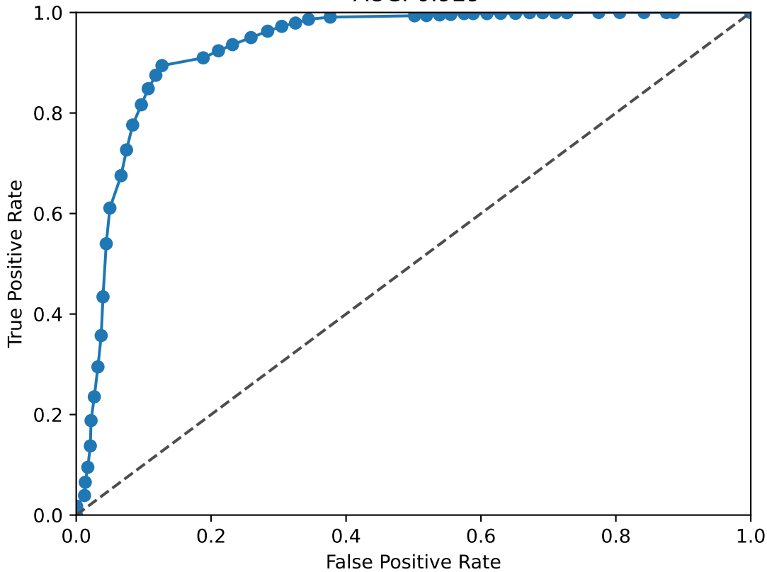
EPCAM ROC Curve AUC: 0.929
