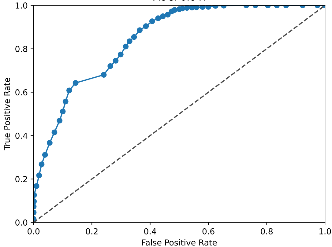
ETS1 ROC Curve AUC: 0.847
