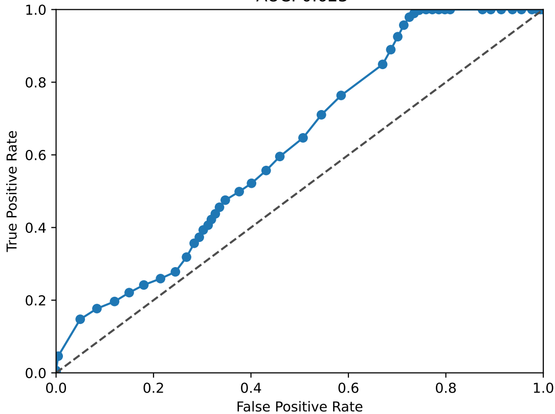
FOXO3 ROC Curve AUC: 0.623
