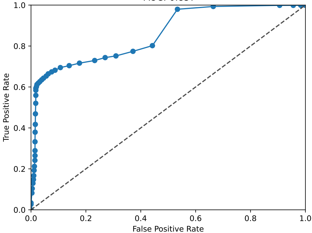
RUNX1 ROC Curve AUC: 0.857
