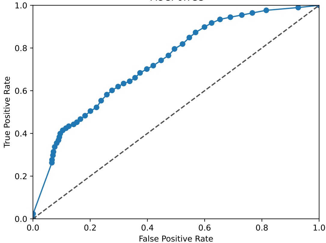
ASCL1 ROC Curve AUC: 0.735
