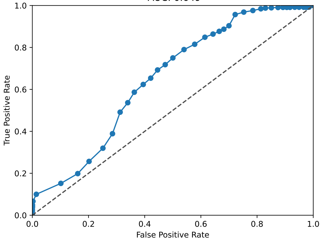
EGR1 ROC Curve AUC: 0.649
