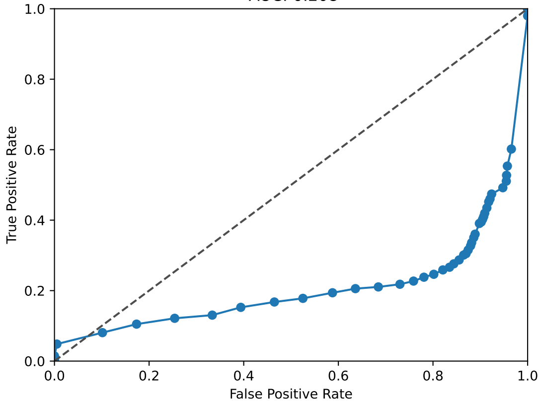
ETS1 ROC Curve AUC: 0.208
