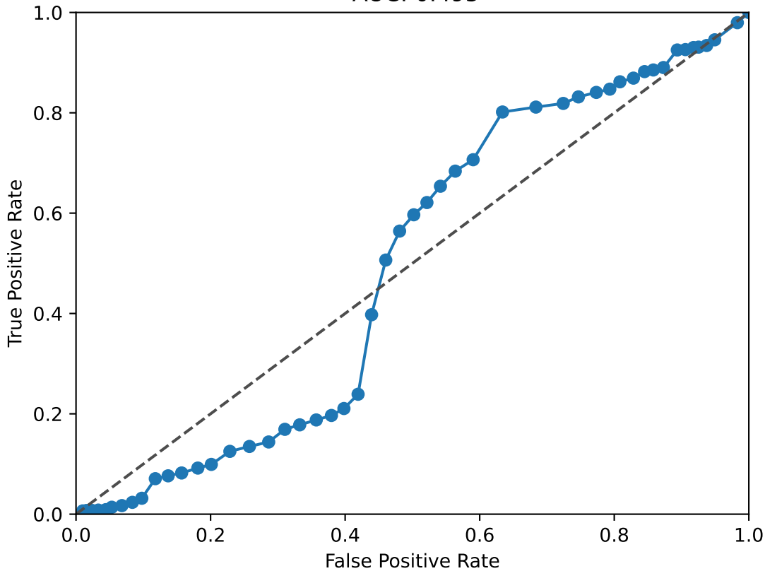
HES1 ROC Curve AUC: 0.495
