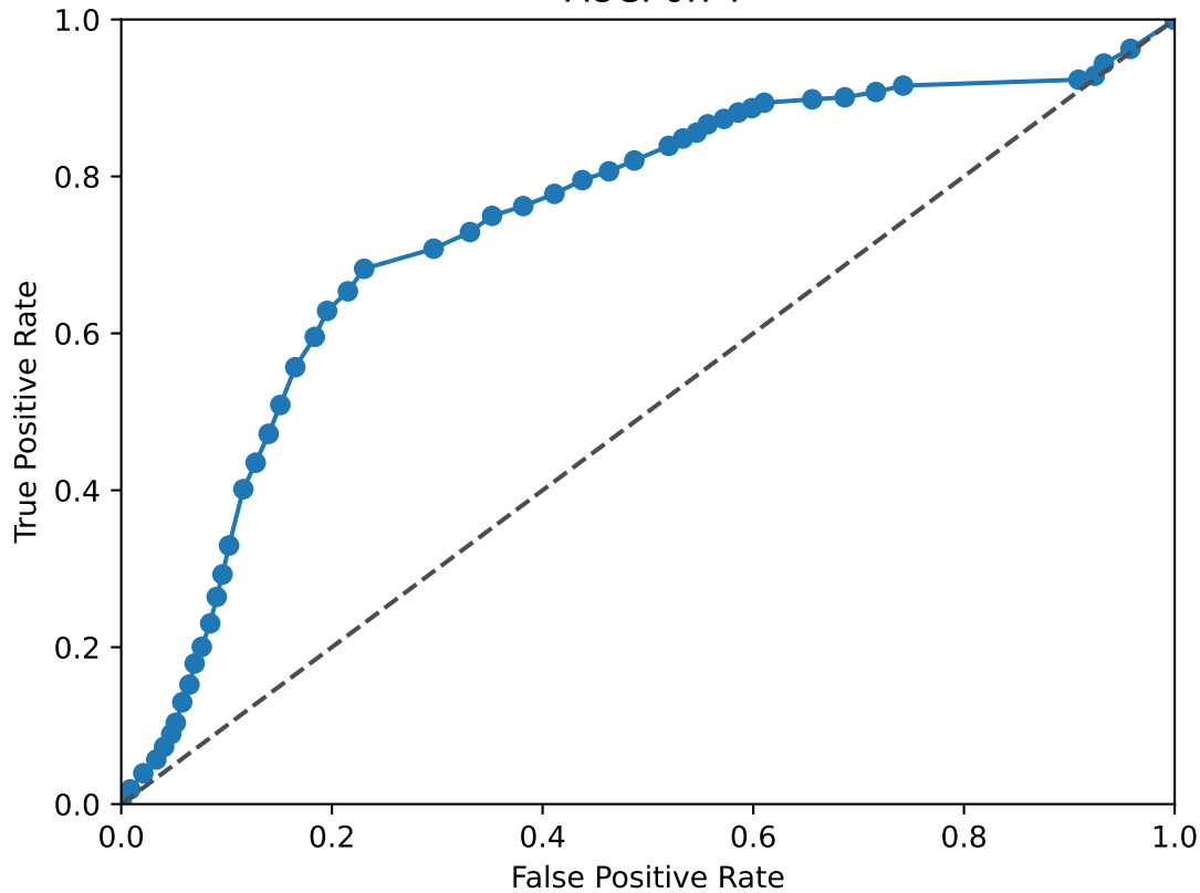
HSF2 ROC Curve AUC: 0.74
